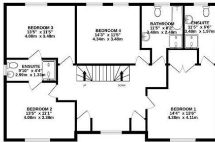
1ST FLOOR 1018 sq.ft. (94.6 sq.m.) approx.
